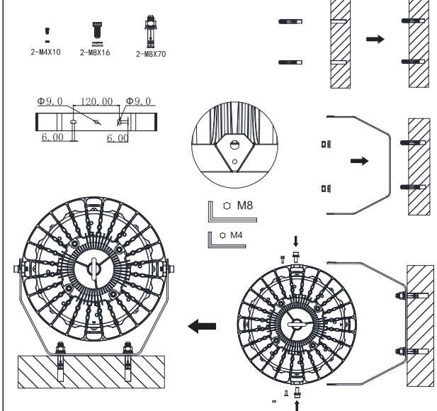
3- Bracket Mount
